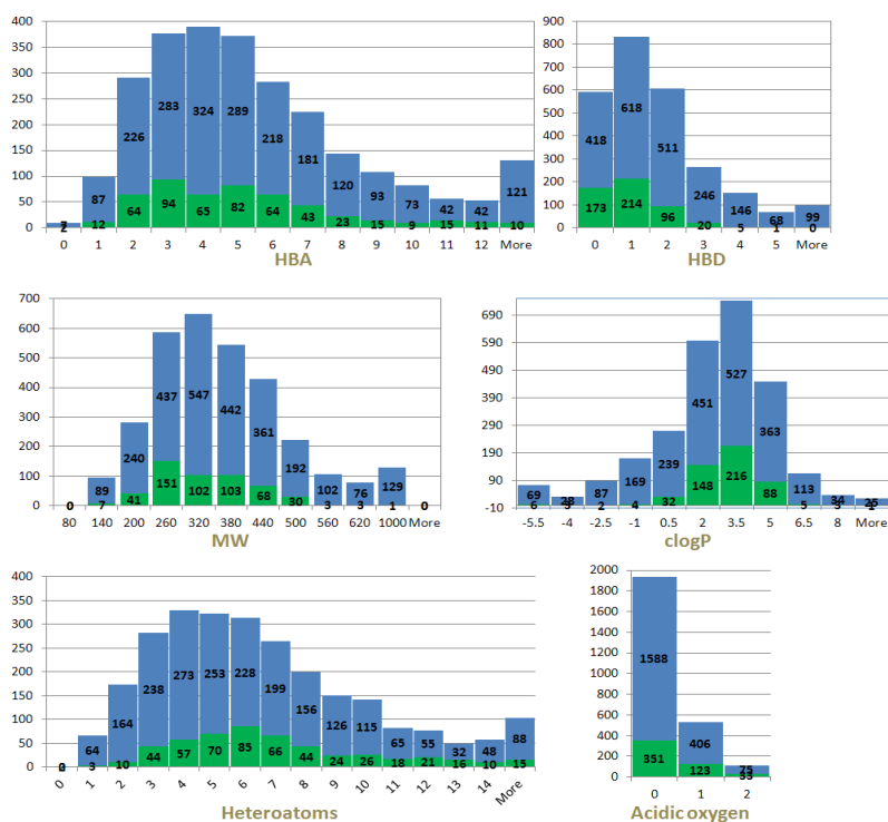
Fig. 1. Distribution of structural parameters (numbers of hydrogen bond acceptors ( HBA ) and donors ( HBD ), heteroatoms as well as acidic oxygen atoms, and of molecular weight ( MW )) in data sets of herbicides (green) and drugs (blue). Numbers of compounds within each bin are denoted.
