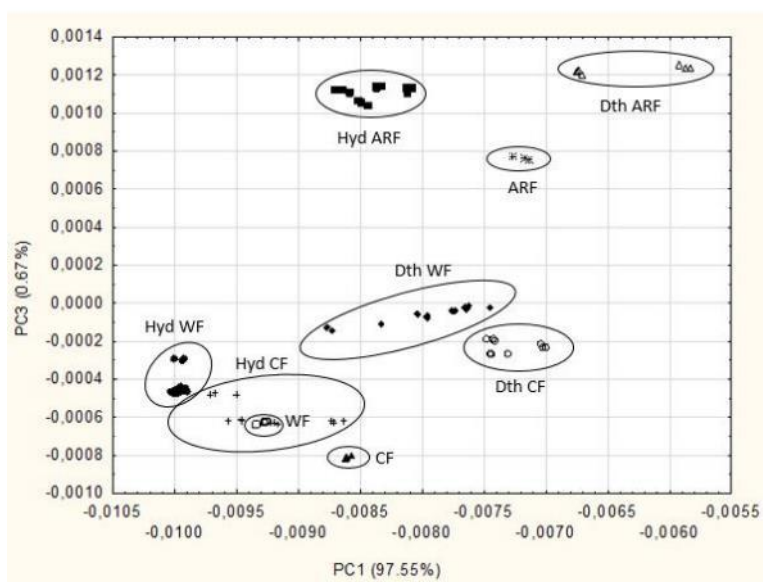
Figure 2. PCA score plot in the case of the untreated (▲: CF; □: WF; #: ARF), dry-thermal treated (◆: Dth WF; ○: Dth CF; △: Dth ARF) and hydrothermal-treated (●: Hyd WF; +: Hyd CF; ■: Hyd ARF) samples based on D2OD 8/0 nm spectra (CF = cake flour, WF = wheat flour, ARF = aleurone-rich wheat flour).
