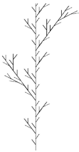
(b) n = 3
