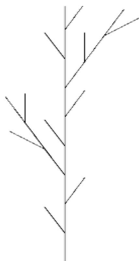
(a) n = 2
