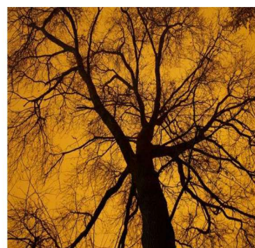
(c) Drvo
