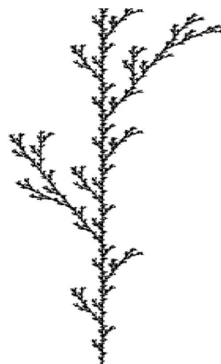
(c) n = 4
