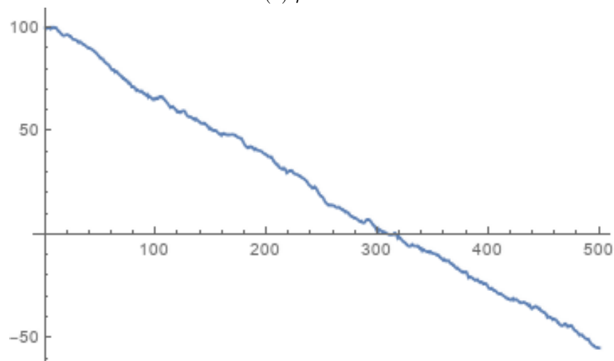
(b) \mu = -0.3
