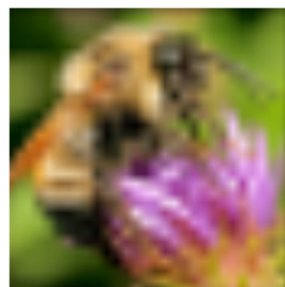
Bilinear interpolation
