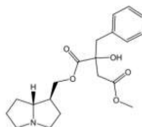
phalaenopsin L (2)
