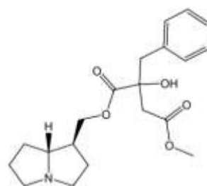
phalaenopsin L (2)
