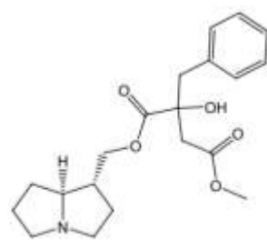
phalaenopsin (1)
