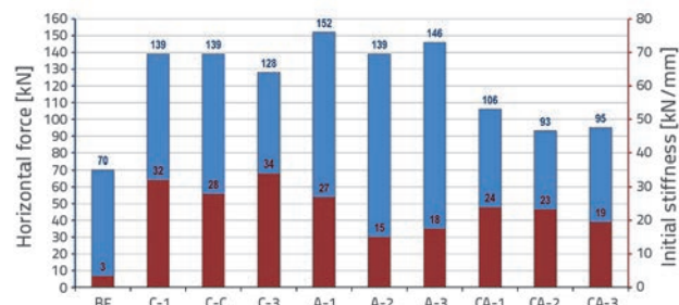
Figure 4. Ultimate load and initial stiffness of bare steel frame (BF), frames infilled with perforated clay blocks (C- i ), AAC blocks (A- i ) and combined infill (CA- i )
