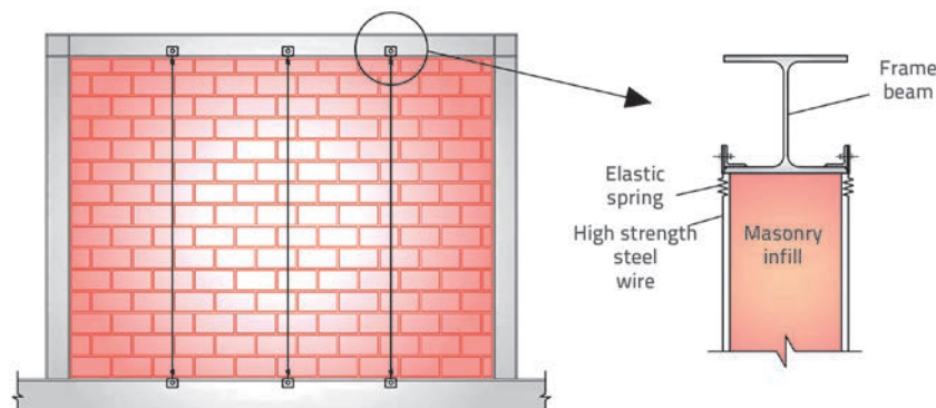
Figure 7. Example of preventing of out-of-plane failure
