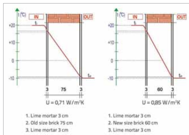
Figure 2. Typical external walls before 1900
