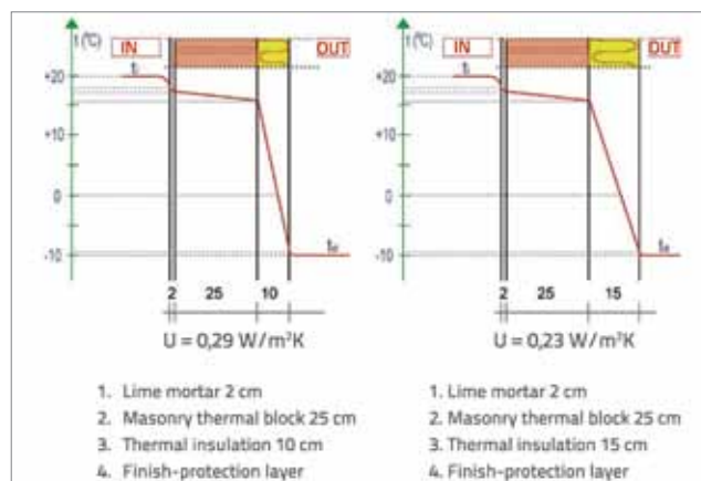
Figure 7. Typical external walls since 2001 to date
