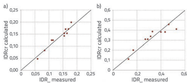
Figure 17. Comparison of experimental results and analytical predictions
