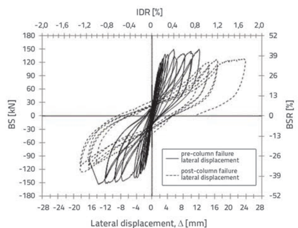
Figure 15. Hysteresis loops of specimen O2\_cpm
