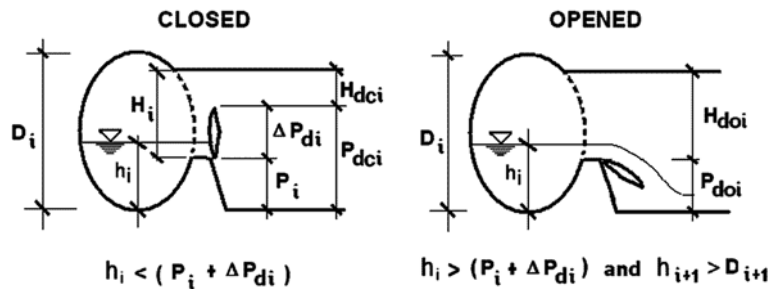
Figure 9 Operational phases of the stormwater overflow "i", operated by a movable watergate Slika 9. Operativne faze preljeva "i" upravljanog s pokretnom ustavom
