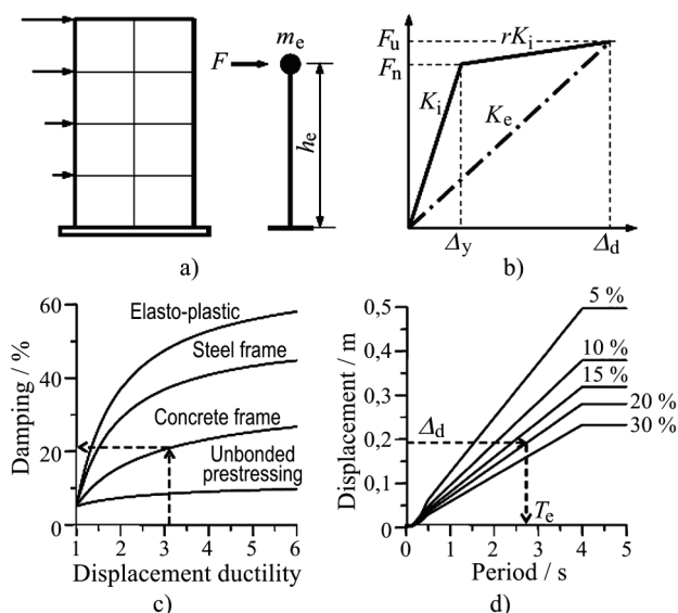
Figure 2 Fundamentals and design method of DDBD [1]
