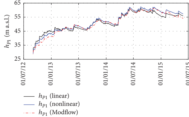
FIGURE 12: Results of the piezometer P1 groundwater level hydrograph (applied coefficients k_{x,y,z} , n_{eff} , n_{tot} of Table 3).
