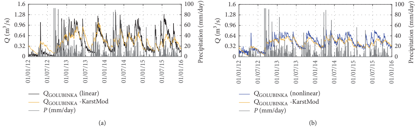
FIGURE 7: Calculated discharges of the Golubinka spring obtained by the KarstMod model simulation, and the linear ( Q = K_m \cdot m ) and nonlinear ( Q = K_m \cdot \text{sqrt}(m) ) approach from the first step of the methodology.
