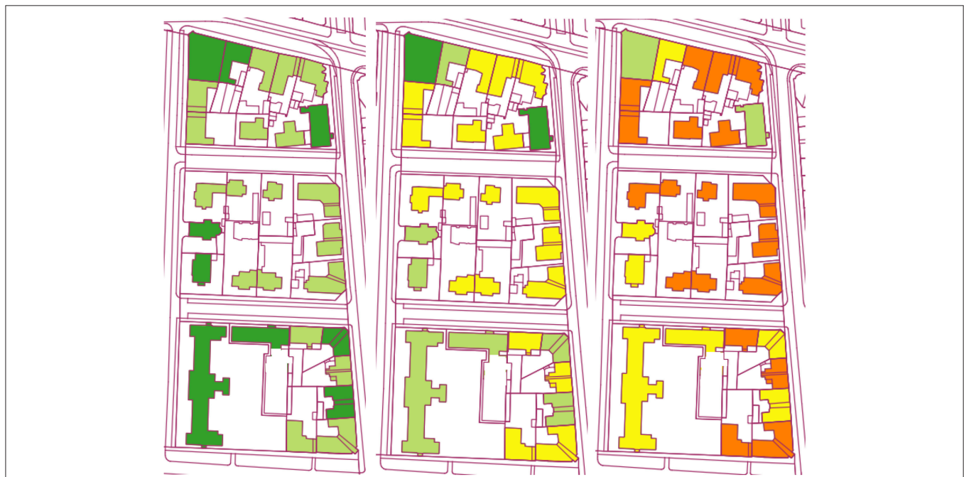
FIGURE 9 | Values of the mean damage grades for three levels of earthquake intensity: (A) VII, (B) VIII, and (C) IX.
