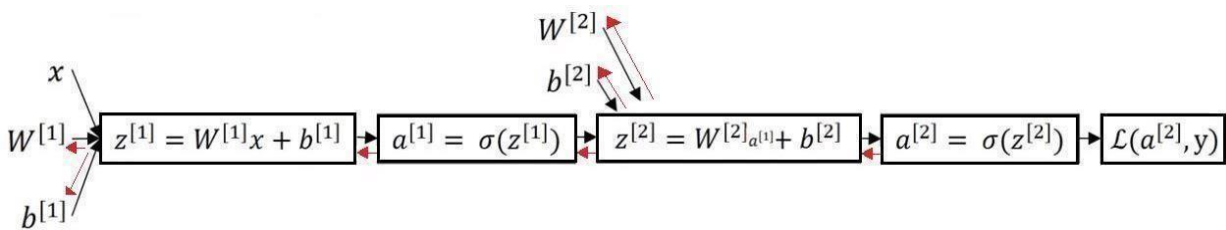
Slika 2.9. Gradient Descent
