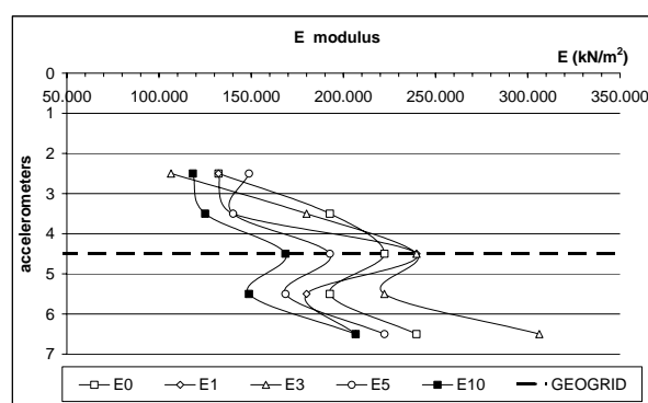
Fig. 1. Measured E modulus distribution around the grid in gravel using P wave propagation method (distance between measuring points is 10 cm, results correspond to zones between them), E_i - E modulus at different displacement ( i - displacement of the grid in millimeters)
