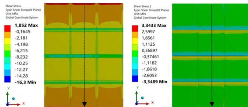
Figure 8 Shear stresses \tau_{xy} (left) and shear stresses \tau_{zx} (right) in model H600-5
