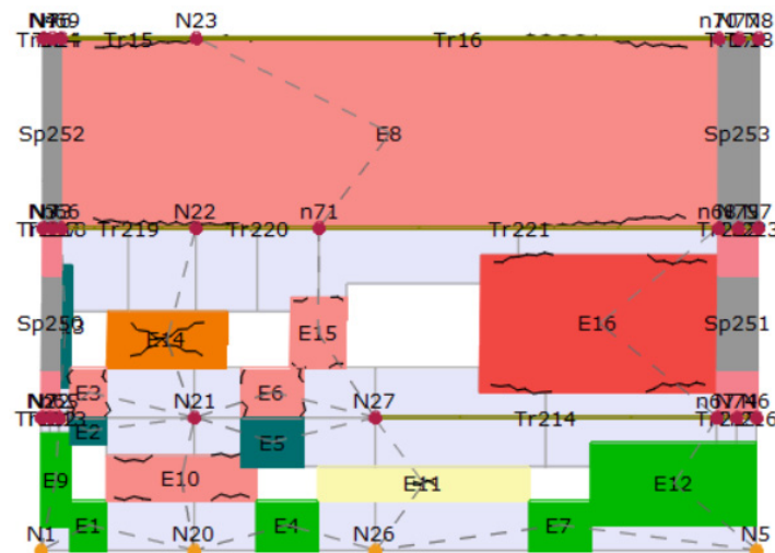
Figure 14. Damage of the wall during analysis no. 11.
