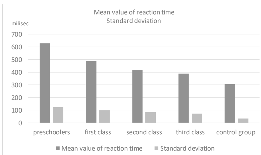
Figure 1. Descriptive Statistics.
