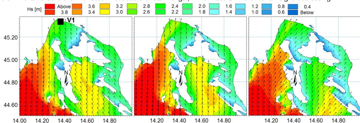
Figure 8 Model H_s fields in the case of a homogenous wind field with a velocity of 18 m/s and transition period from 12 to 18 h of simulation (left – 12 th hour simulation, SSE wind; middle – 15 th hour simulation; right – 18 th hour simulation, SW wind)
