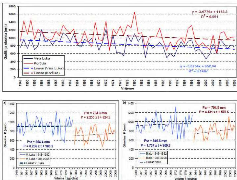
Fig. 6. Application of RAPS method on precipitation data of Korčula, Croatia (1948-2008) (Ljubenkovic, 2011)
