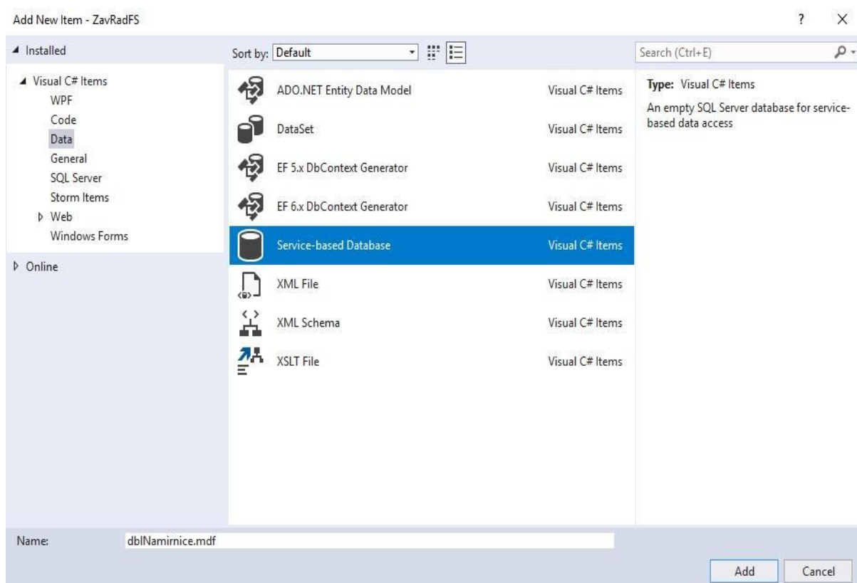
Slika 4.18. Service-based Database
